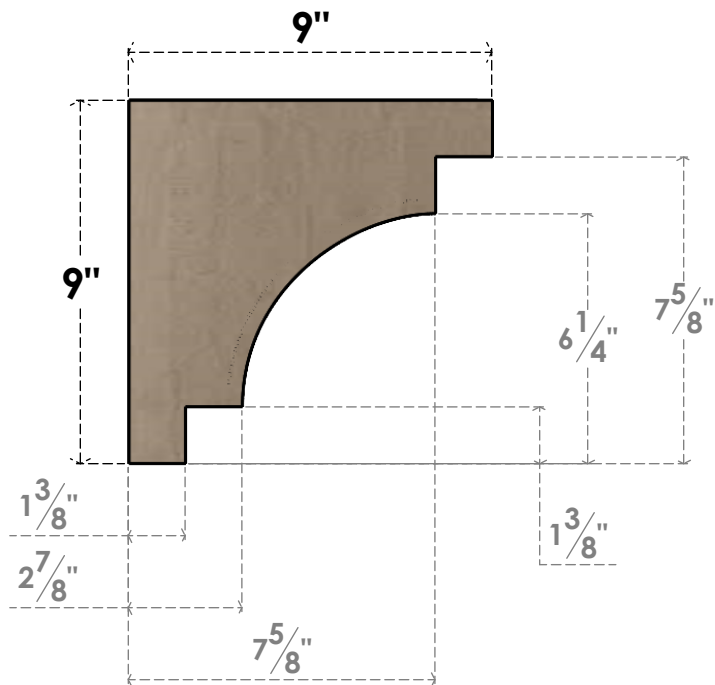
SIDE PROFILE
